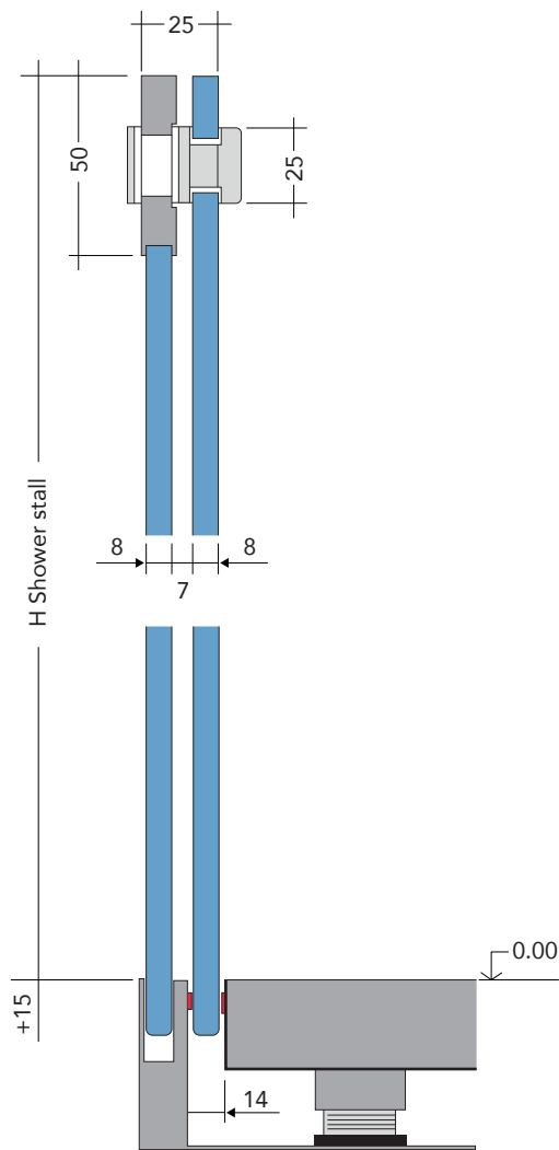
section A-X
