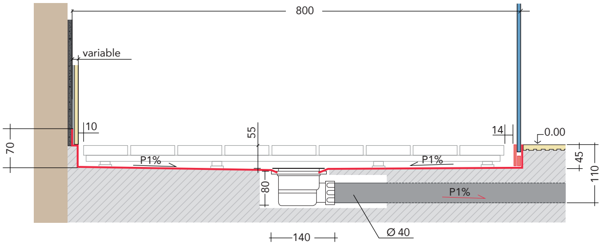
SECTION A-X
