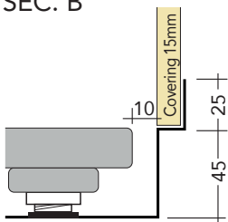
SEC. B
