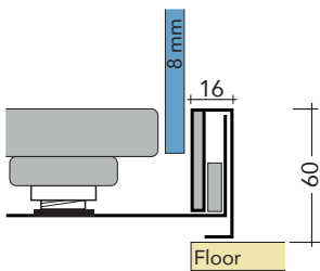
SEC. D
