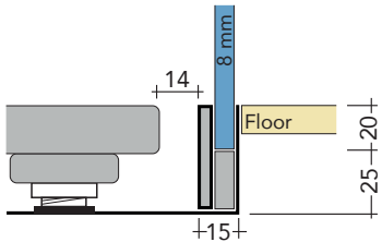
SEC. E
