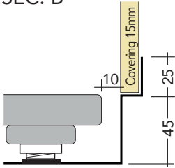
SEC. B
